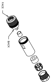
1032-33731: 5 Pin Female Straight Body Connector
