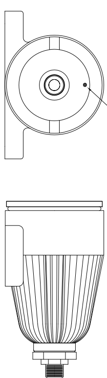
7030-35610-6 CAMERA MCI 50 WATER TIGHT BLACK & WHITE 3.6 MM, FORWARD VIEWING, HIGH RESOLUTION, 600 LINES, 0.0003 LUX, 12 VDC @ 100mA WITH 5 PIN CONNECTOR
